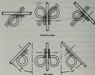
FIGURE 4-96. Proper mounting angle for cable clamps.
